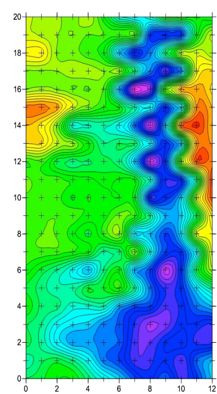
Underground river (2-3m)
